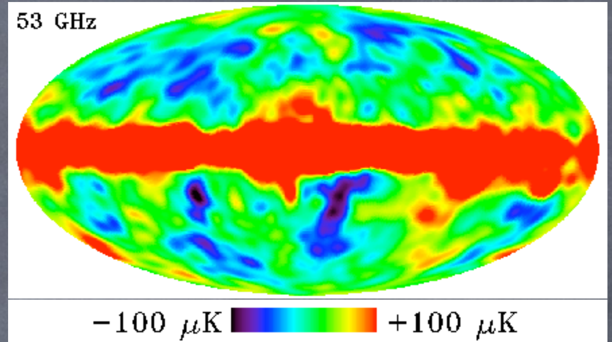
Four-year COBE map of the cosmic microwave background sky.
