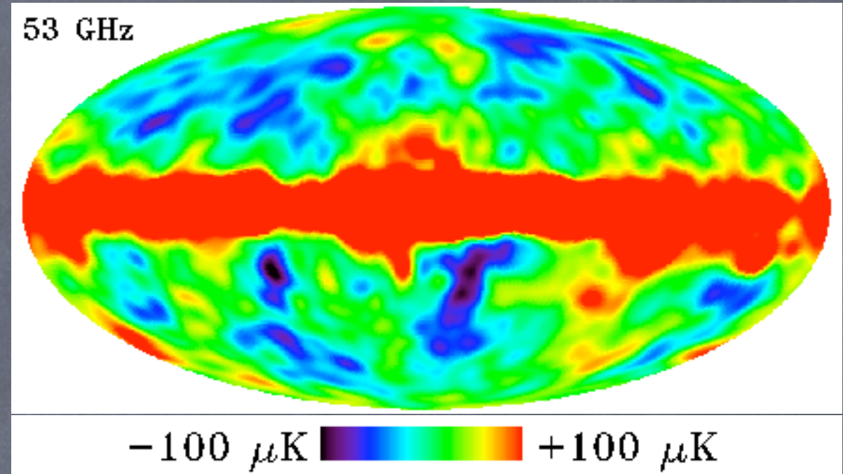
Four-year COBE map of the cosmic microwave background sky.
