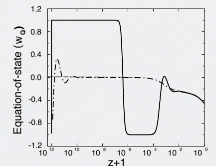
FIG. 1: Examples of the behaviour of the equation of state (here called w_\phi ) for a tracker potential. The thin-dashed line originating at w_\phi = 0 corresponds to the tracker solution. Reproduced from Ref. [18].
